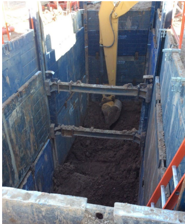
Figure 136: Excavation and Bore Pit
