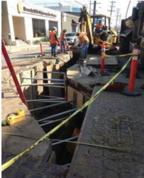
Figure 7: Shoring Installed in Pipeline Trench
