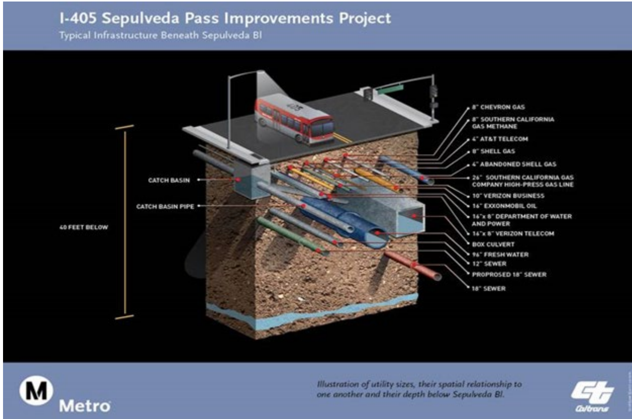
Figure 1: Substructure Example
